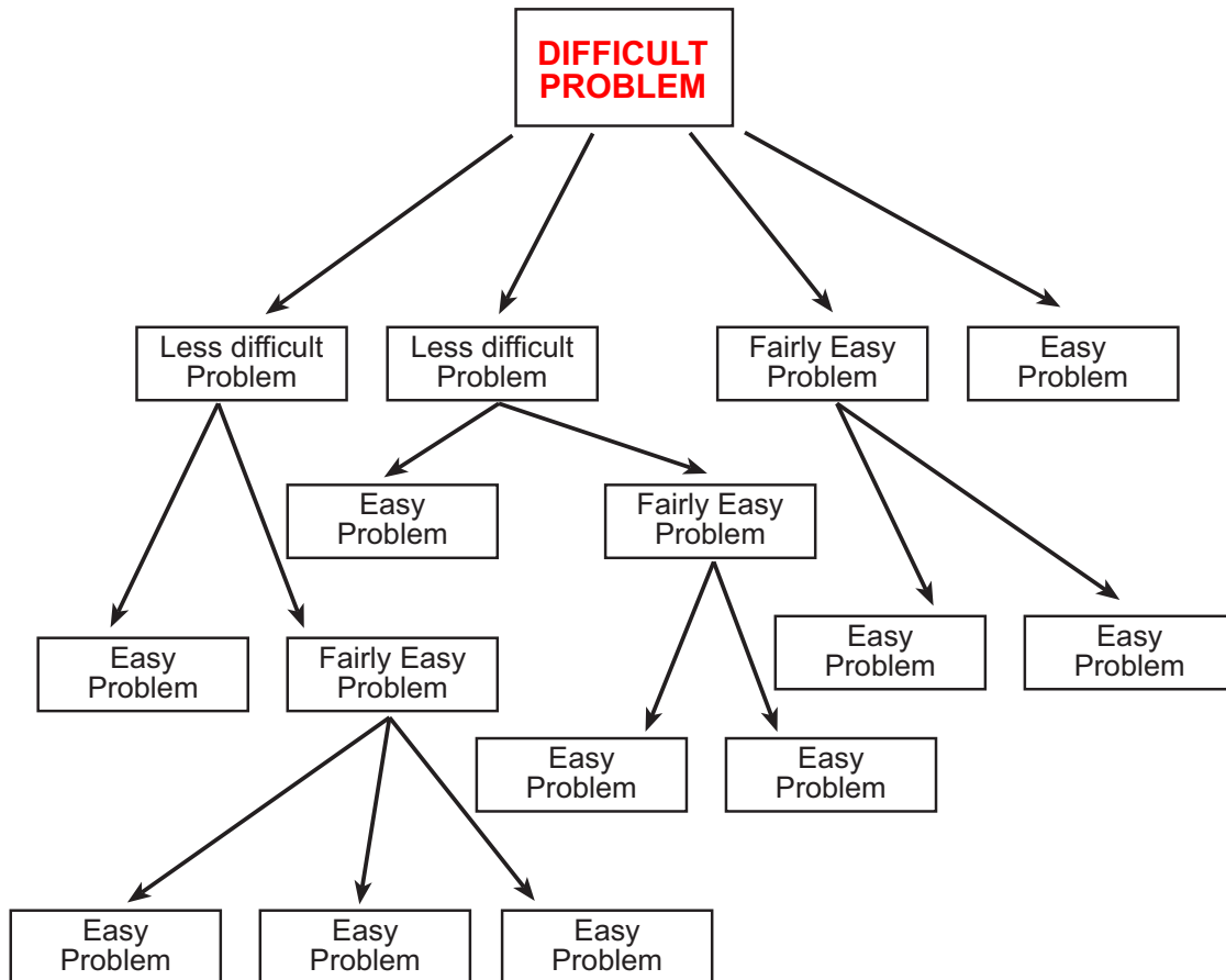
Figure 3.1: Stepwise refinement
